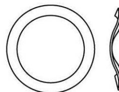
19.5*24.8*0.25mm (#51) *2
